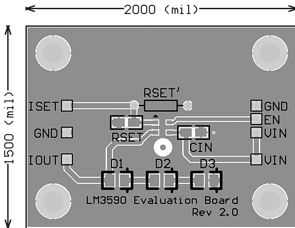
Figure 2. Top Layer, Top View
