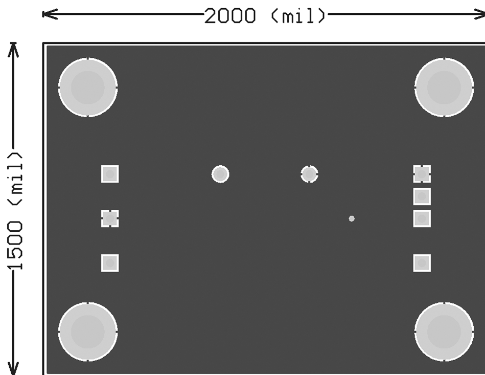
Figure 3. Bottom Layer, Top View (unmirrored)
