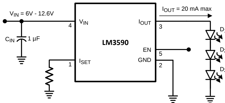
Figure 1. Evaluation Board Schematic
