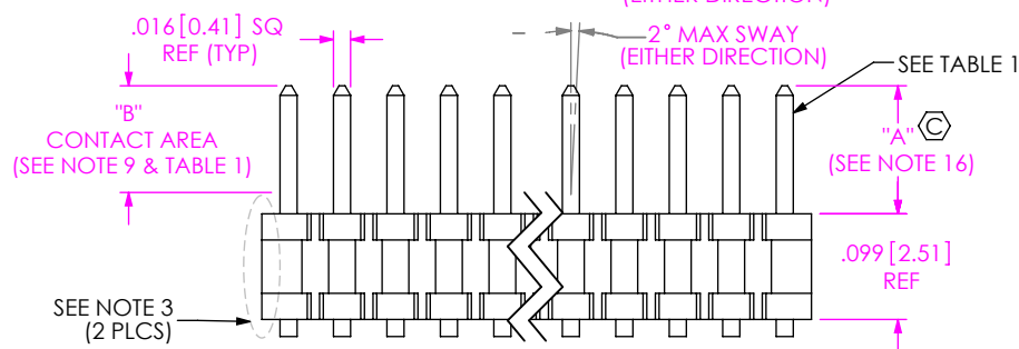
FIG 1 FTSH-1XX-XX-XXX-DV SHOWN
