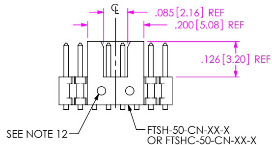
FIG 2 -K OPTION (LEAD STYLE -01 ONLY) (DIFFERENT AS SHOWN, OTHERWISE SAME AS FIG 1) (POSITION 13, 17, 20 & 25 AVAILABLE WITH -EXX OPTION)
