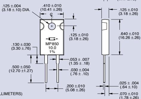
Figure 3 TO-220 Style MP850
