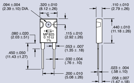
Figure 2 TO-126 Style MP825
