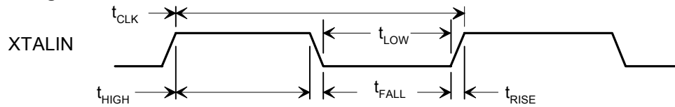
Clock Timing
