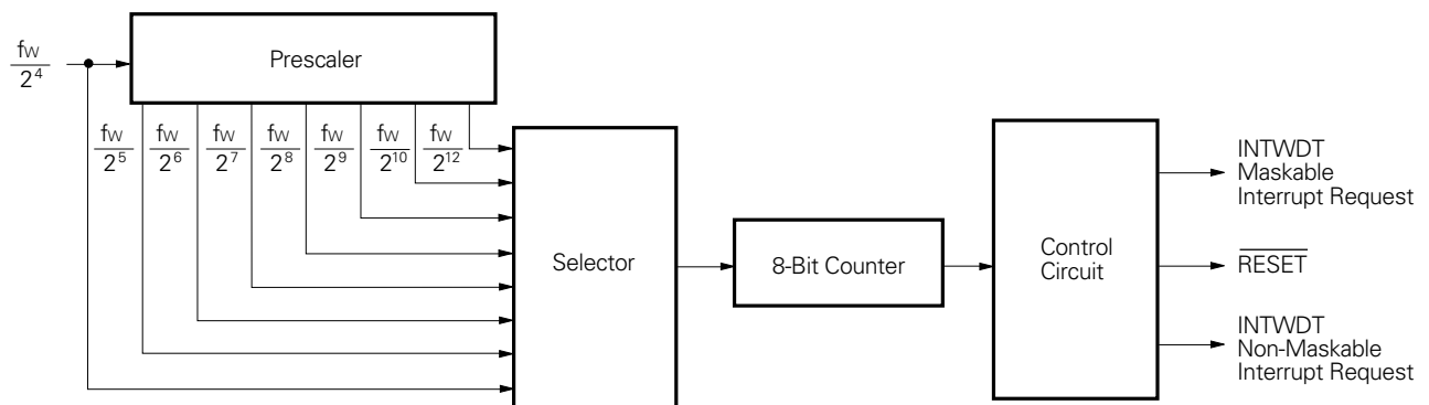
Fig. 5-4 Watchdog Timer Block Diagram
