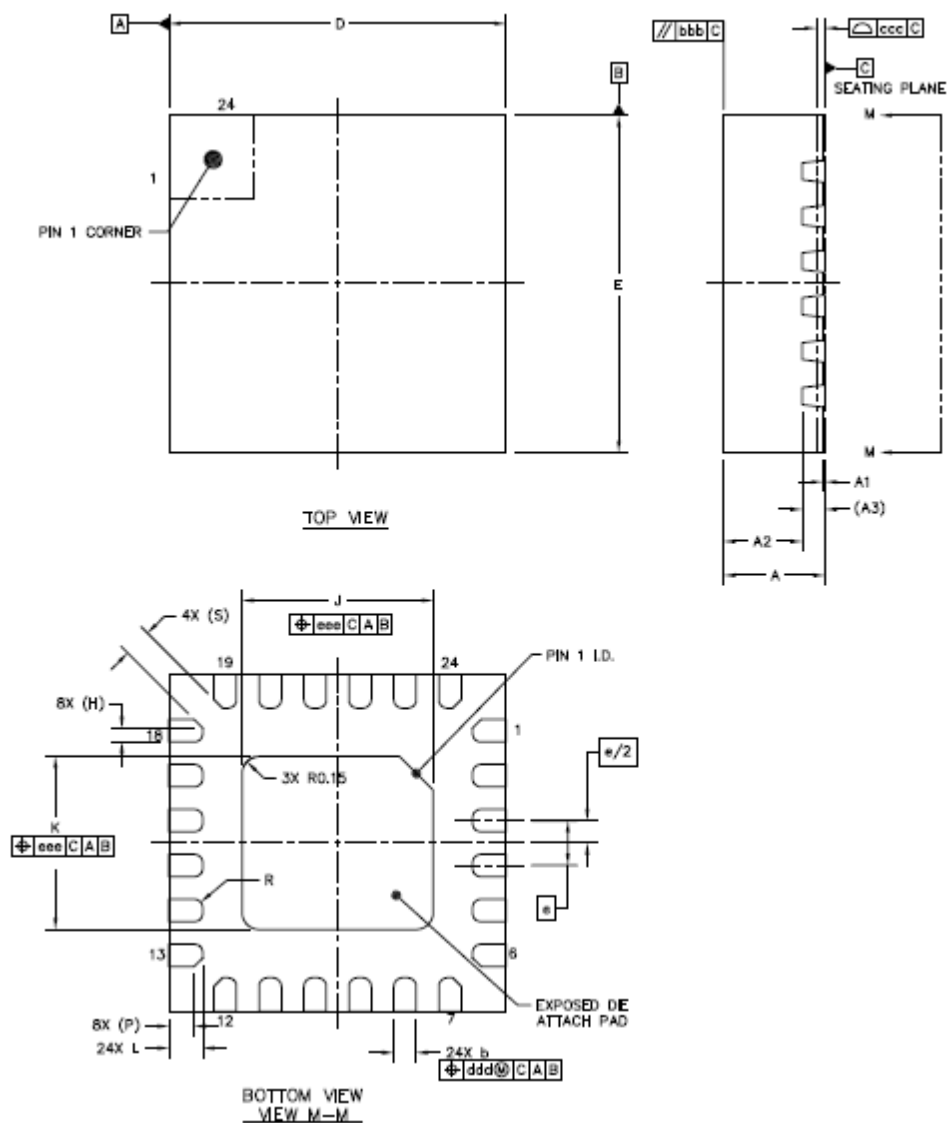
Figure 13. Package Dimensions
