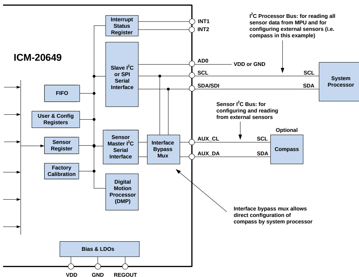
Figure 6. ICM-20649 Solution Using I 2 C Interface
