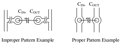
Figure 11-11. Pattern Example
