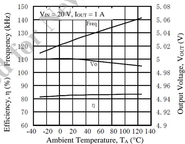
Figure 13-12. Temperature Characteristic
