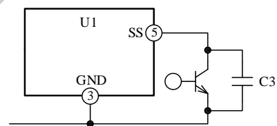
Figure 10-8. Rising Delay Time Setting
