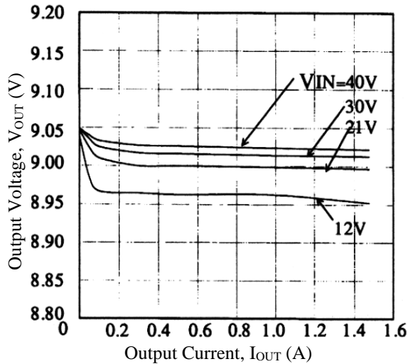
Figure 13-17. Load Regulation
