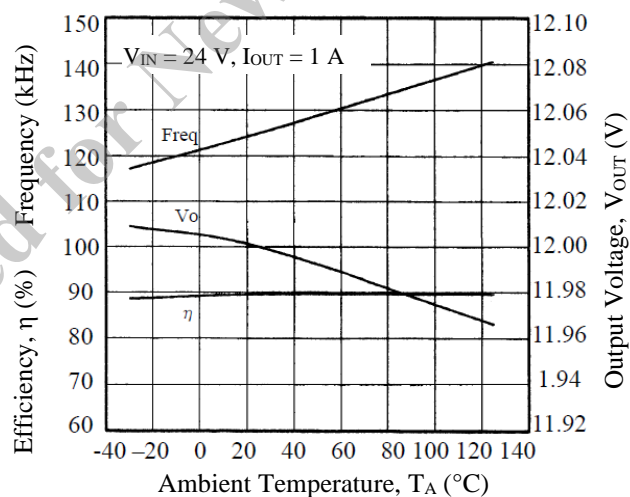
Figure 13-24. Temperature Characteristic
