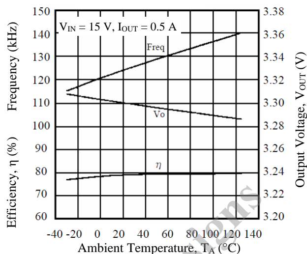
Figure 13-6. Temperature Characteristic
