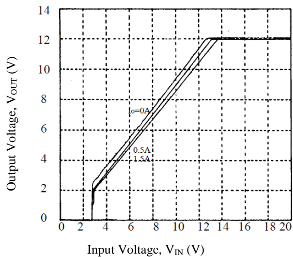
Figure 13-21. Rising Characteristics
