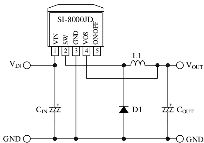
Figure 7-1. Typical Application
