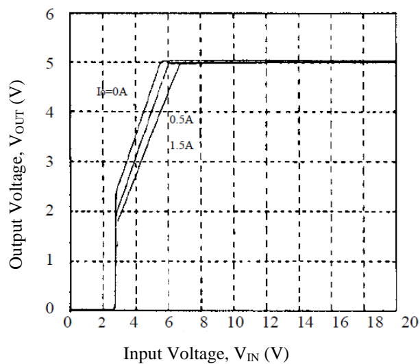
Figure 13-9. Rising Characteristics
