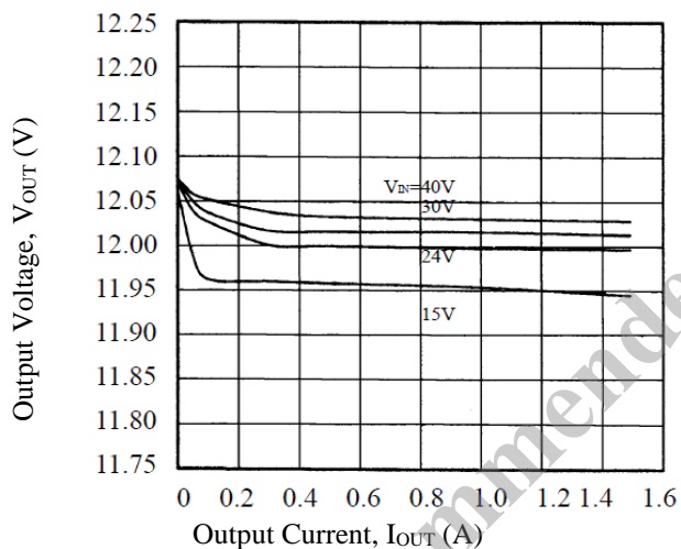
Figure 13-23. Load Regulation
