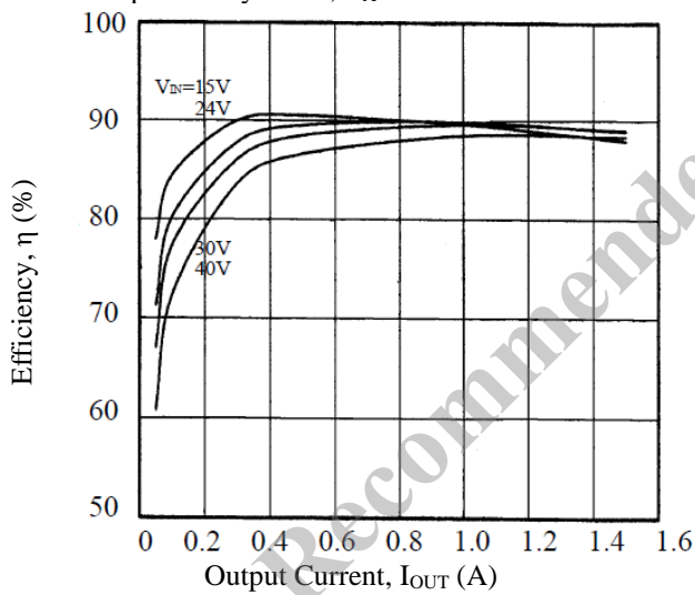
Figure 13-19. Efficiency
