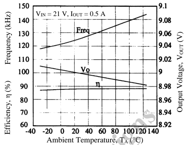
Figure 13-18. Temperature Characteristic
