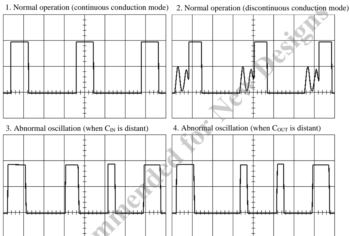
Figure 11-12. Waveform Examples
