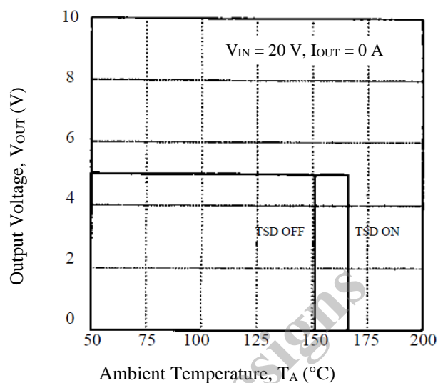
Figure 13-10. Thermal Shutdown Characteristics
