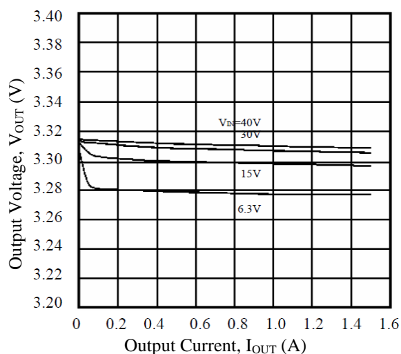
Figure 13-5. Load Regulation
