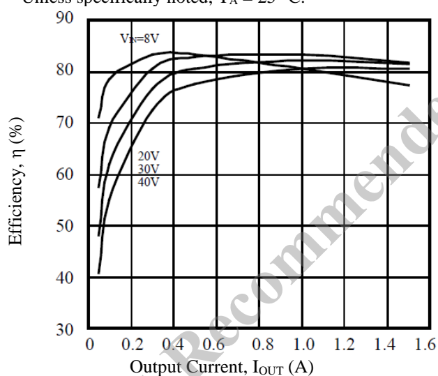
Figure 13-7. Efficiency
