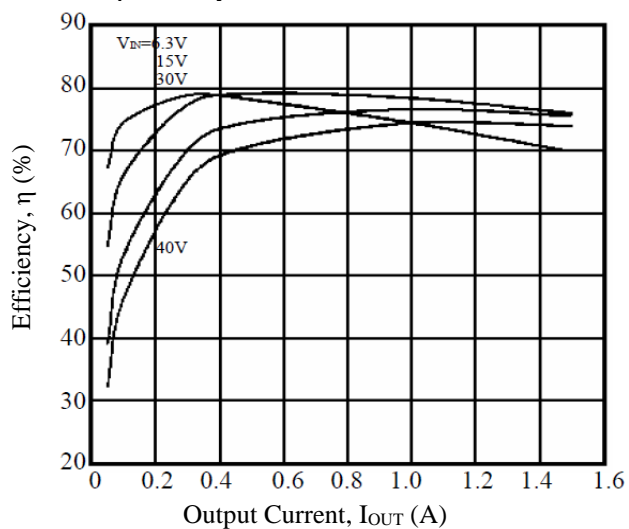
Figure 13-1. Efficiency
