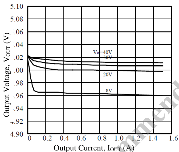
Figure 13-11. Load Regulation
