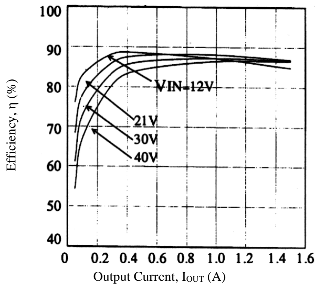
Figure 13-13. Efficiency
