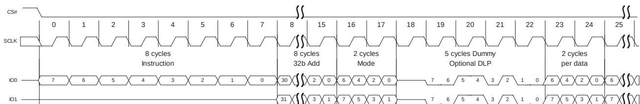
Figure 10.46 DDR Dual I/O Read Initial Access (4-byte Address, BEh or BDh [ExtAdd=1], EHPLC= 01b)
