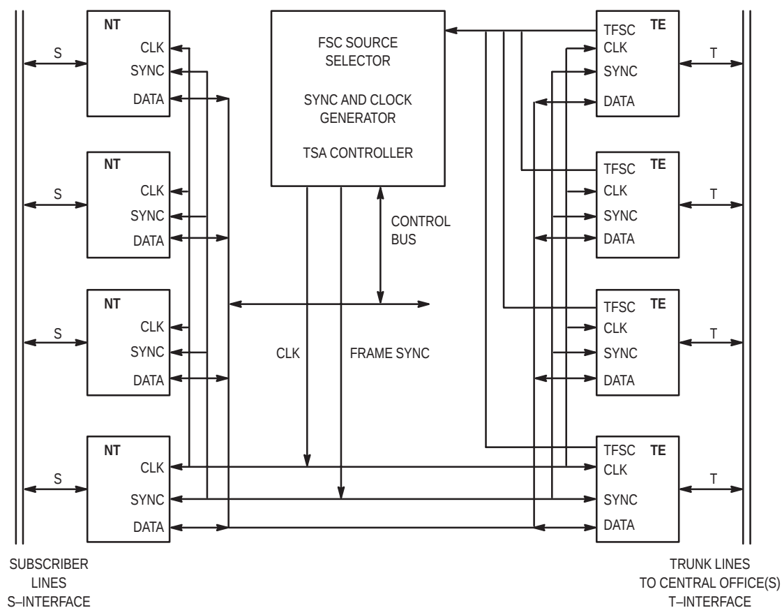
Figure 13–3. NT2 Architecture
