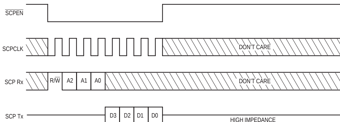
Figure 5–1. Serial Control Port Nibble Register Read Operation
