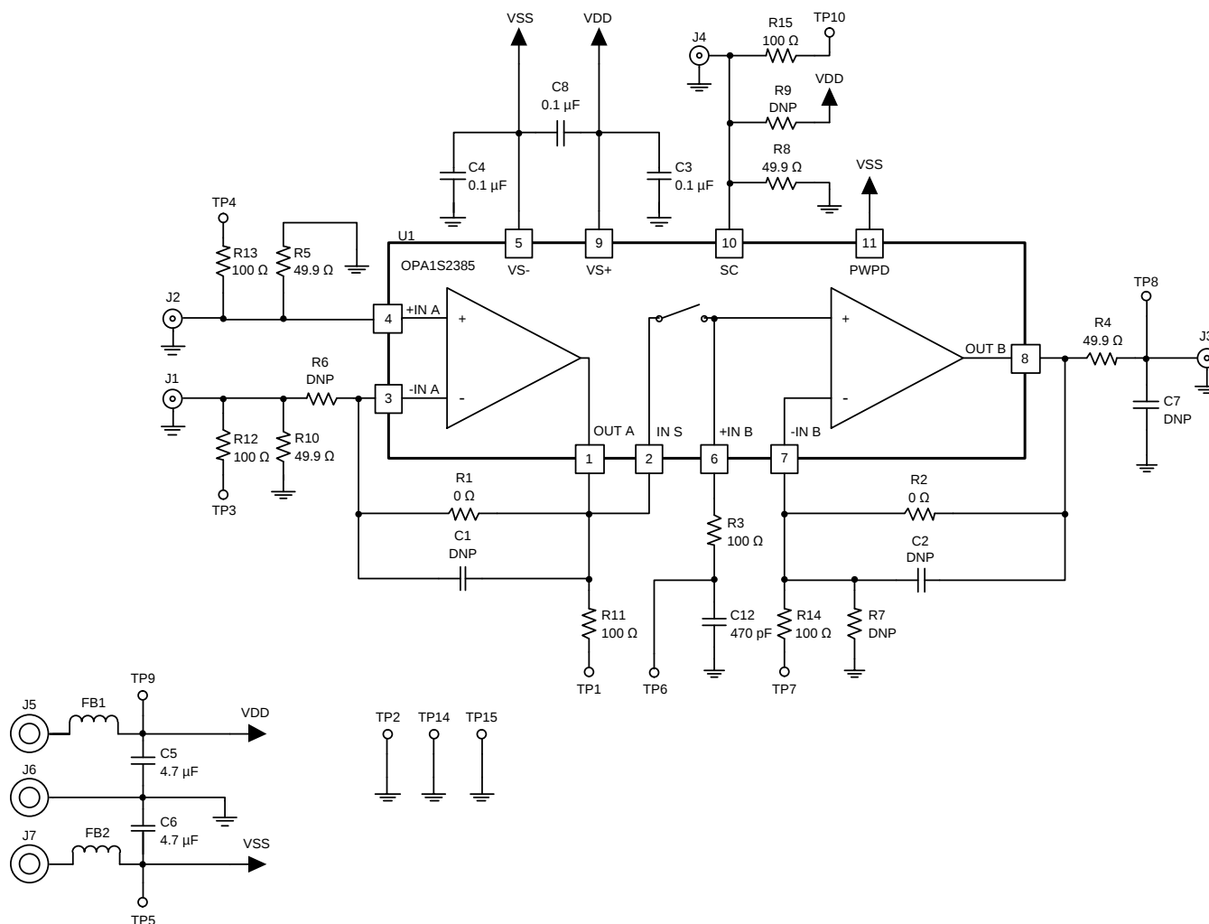
Figure 2. OPA1S238xEVM Schematic
