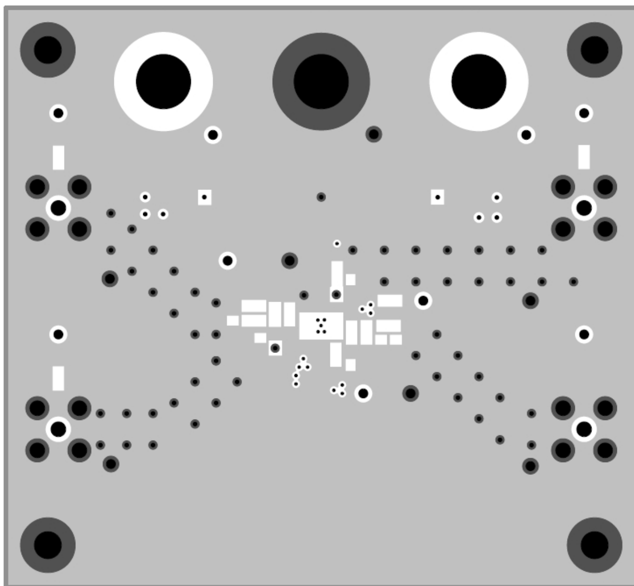
Figure 4. Layer 2 (Ground)
