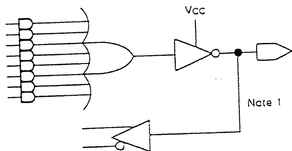
Combinatorial Output Active Low
