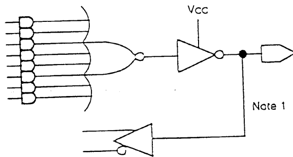
Combinatorial Output Active High
