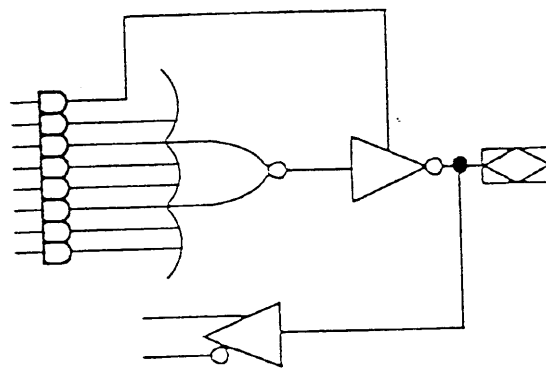
Combinatorial I/O Active High
