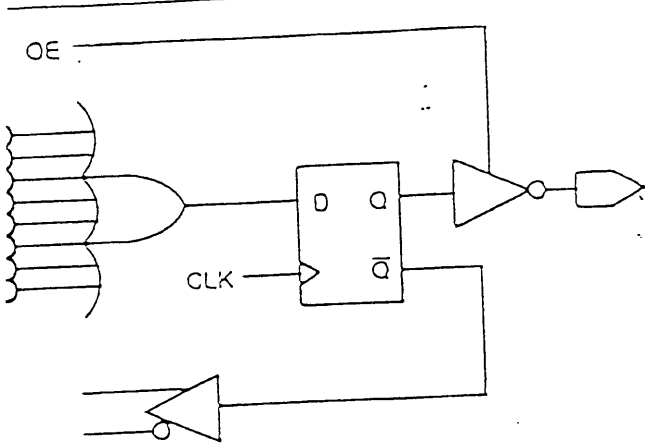
Registered Active Low
