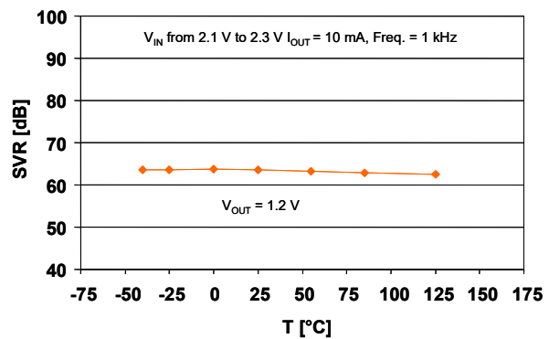
Figure 19. Supply voltage rejection vs. temperature ( V_{OUT} = 1.2\text{ V} )
