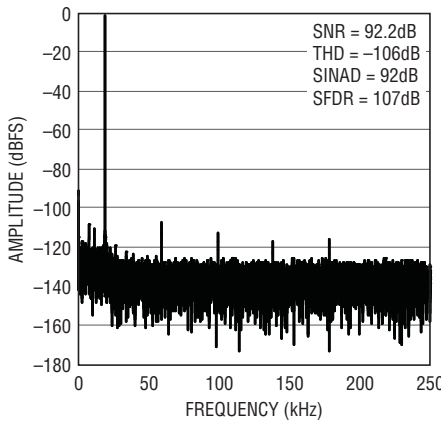
32k Point FFT f_s = 500\text{Ksps} , f_{\text{IN}} = 20\text{kHz}
