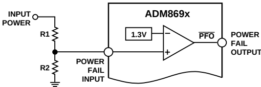
Figure 7. Power Fail Comparator
