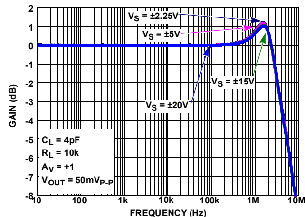
FIGURE 46. GAIN vs FREQUENCY vs SUPPLY VOLTAGE
