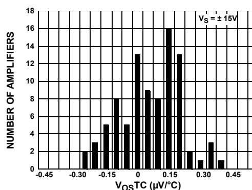
FIGURE 2. V_{OS} TEMPERATURE COEFFICIENT ( V_{OS\text{TC}} )
