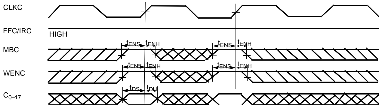
Port C Word Write Cycle Timing for FIFO2 (CY Standard and FWFT Modes)
