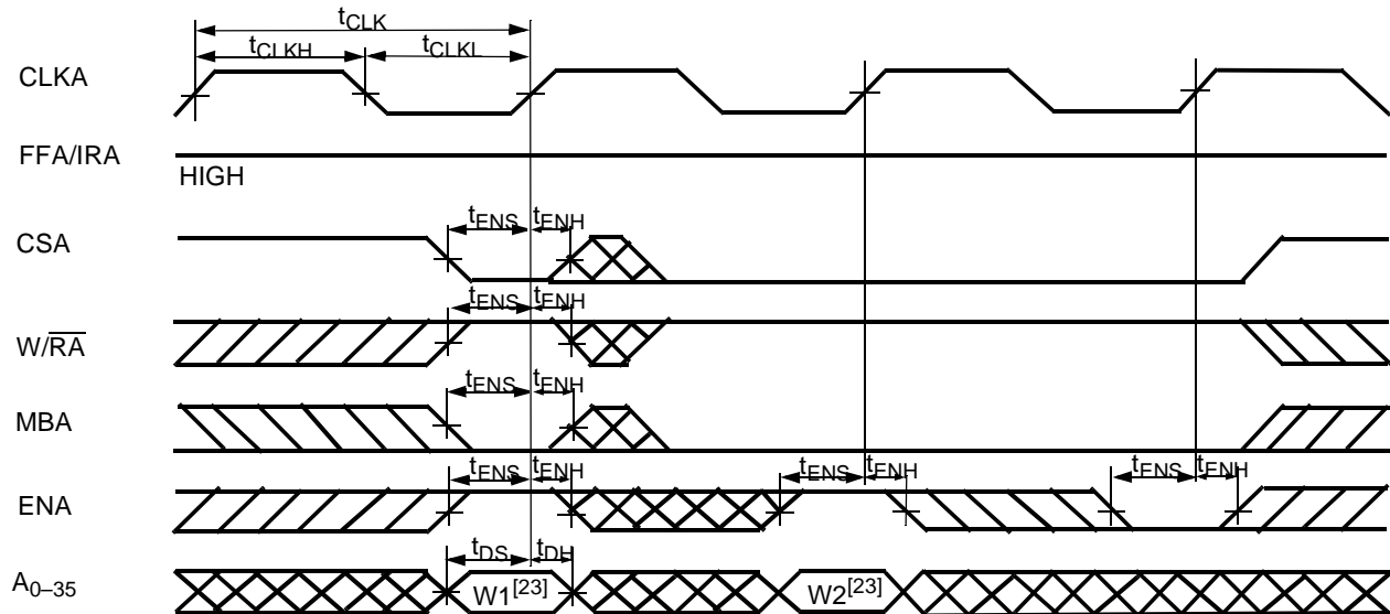
Port A Write Cycle Timing for FIFO1 (CY Standard and FWFT Modes)
