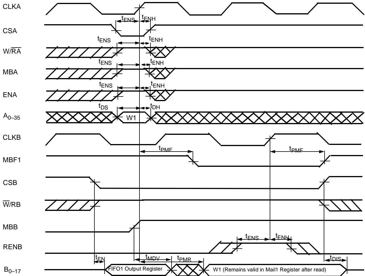
Timing for Mail1 Register and MBF1 Flag (CY Standard and FWFT Modes) [56]
