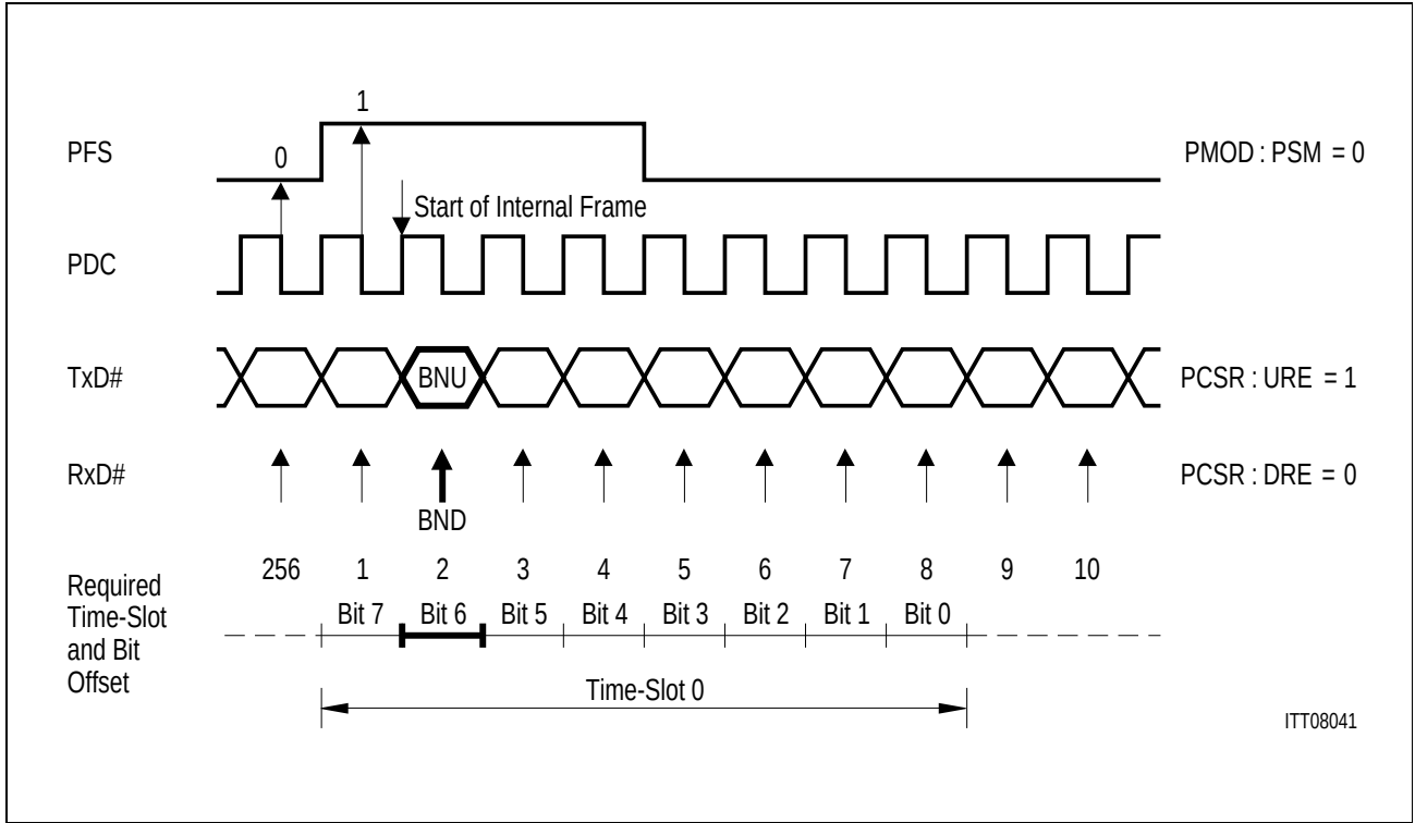
Figure 26 Timing PCM Frame Offset for Example 1
