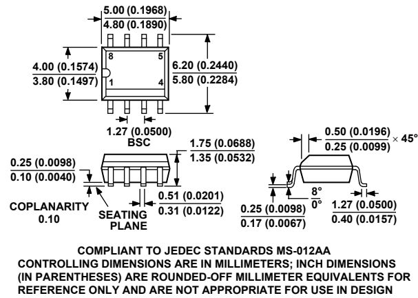
Figure 24. 8-Lead Standard Small Outline Package [SOIC] (R-8) Dimensions shown in millimeters and (inches)
