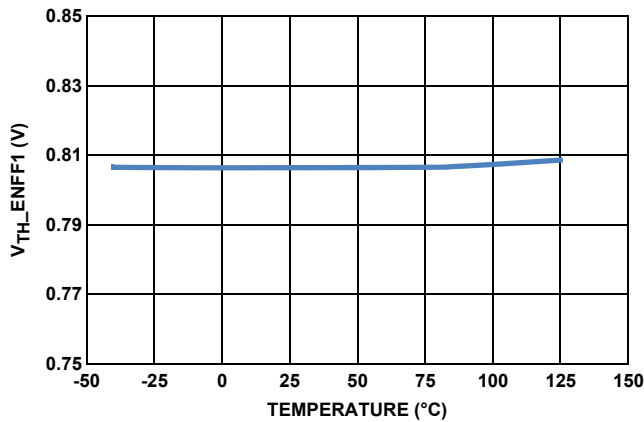
FIGURE 5. V_{EN}/V_{FF1} ENABLE THRESHOLD vs TEMPERATURE
