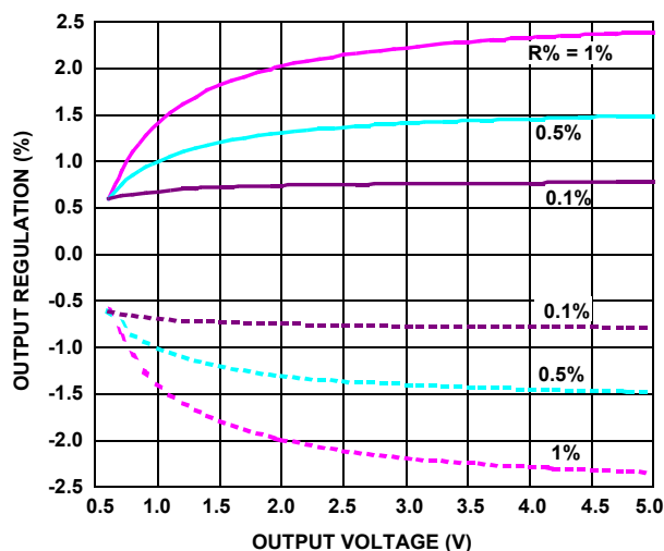
FIGURE 32. OUTPUT REGULATION WITH DIFFERENT RESISTOR TOLERANCE FOR Ref\% = \pm 0.6\%
