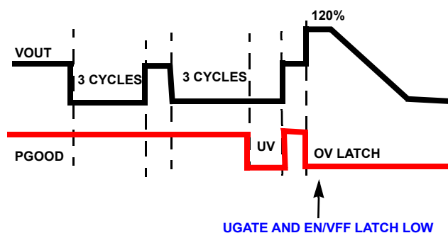
FIGURE 18. PGOOD TIMING UNDER UV AND OV
