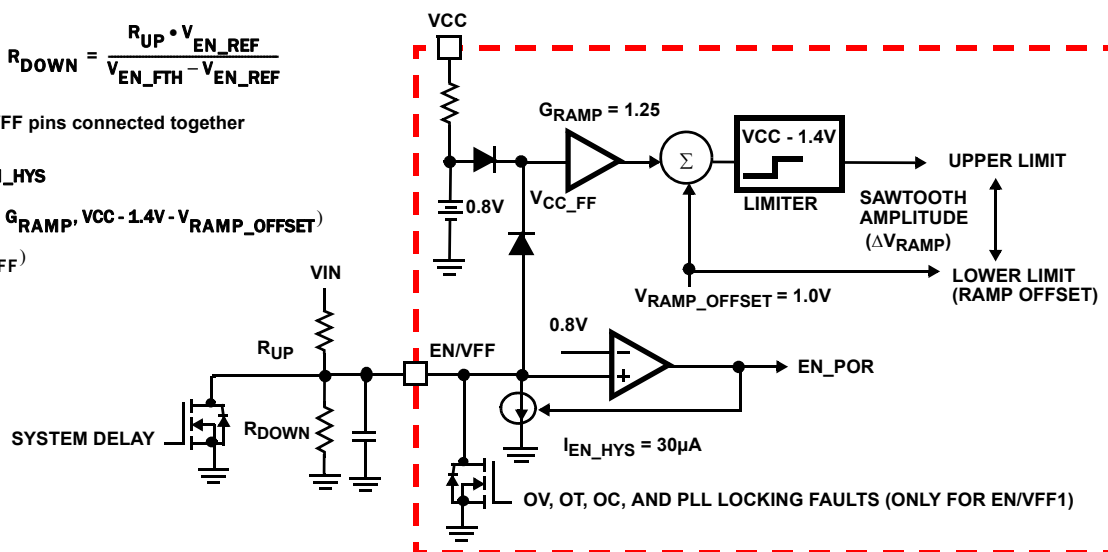
FIGURE 11. SIMPLIFIED ENABLE AND VOLTAGE FEEDFORWARD CIRCUIT
