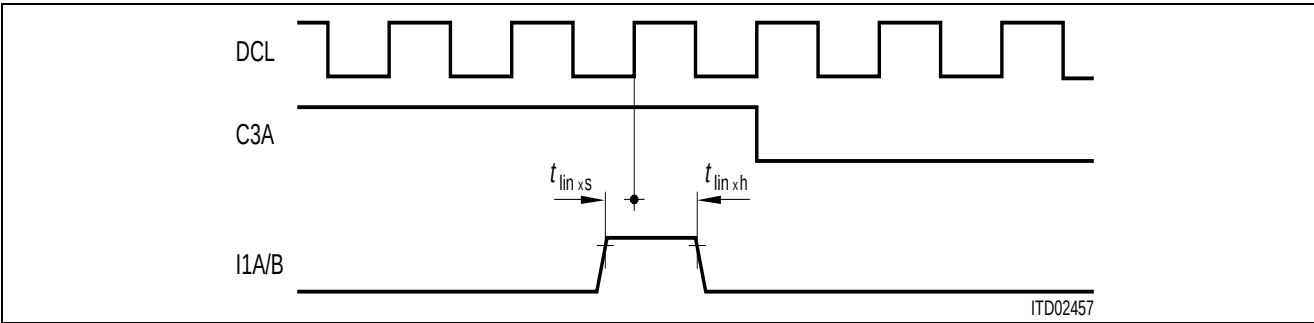
IOM®-2 Interface, DCL = 4096 kHz (eight channels per frame)
