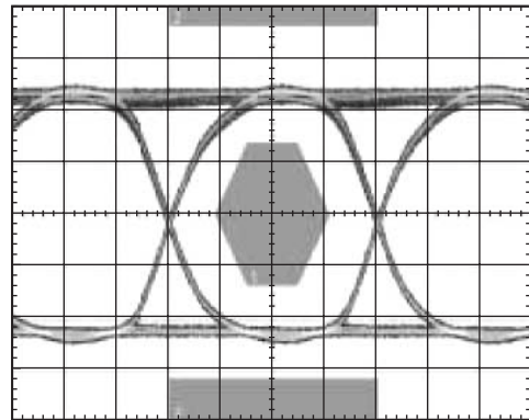
Figure 9. A 1.244 Mbps Optical Eye. Temperature at 85°C. Average Power = 0 dBm, Extinction Ratio = 10 dBm, PRBS 31 Pattern, 1 Gb Ethernet Mask. Eye Obtained Using a DFB Laser.
