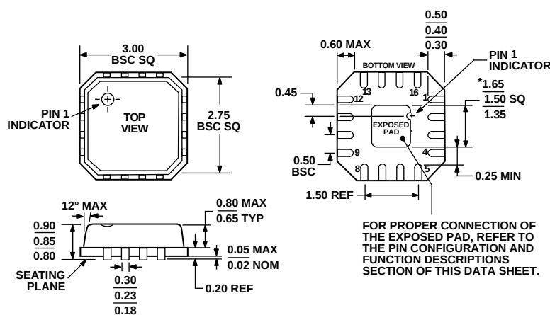
Figure 42. 16-Lead Lead Frame Chip Scale Package [LFCSP_VQ] 3 mm × 3 mm Body, Very Thin Quad (CP-16-3)
