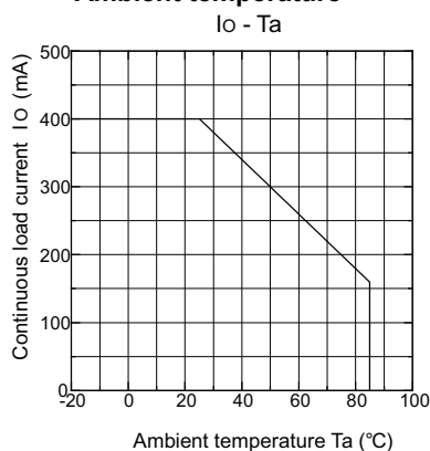
Continuous load current vs. Ambient temperature
