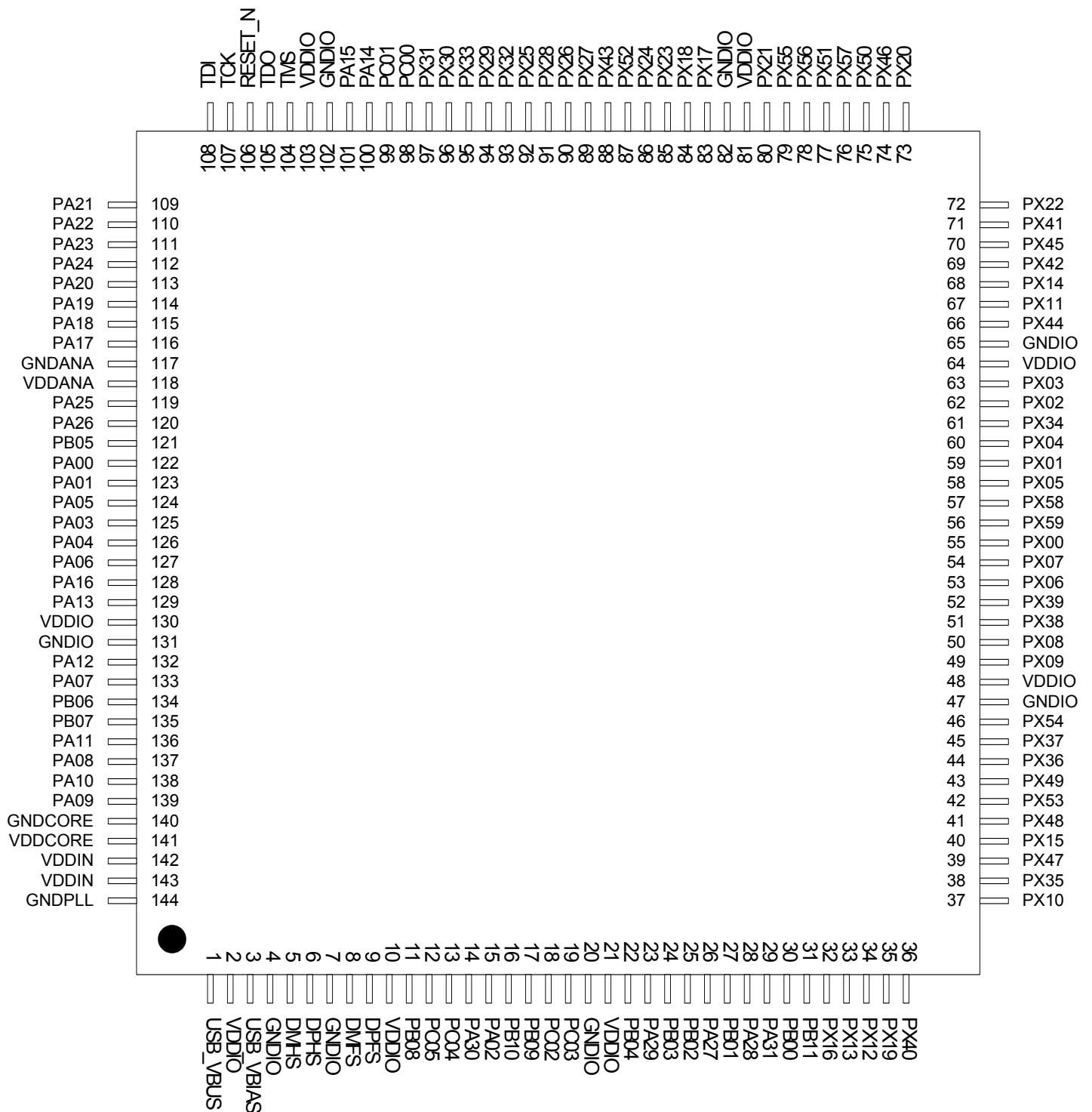
Figure 3-2. LQFP144 Pinout
