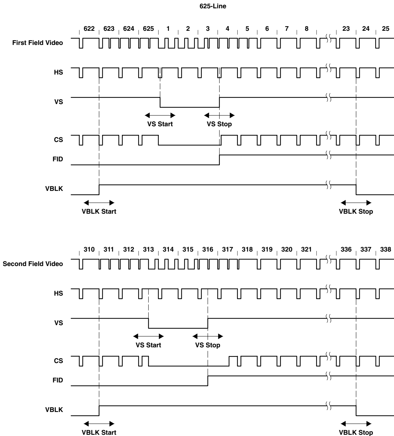
Figure 2–21. Vertical Synchronization Signals for 625-Line System
