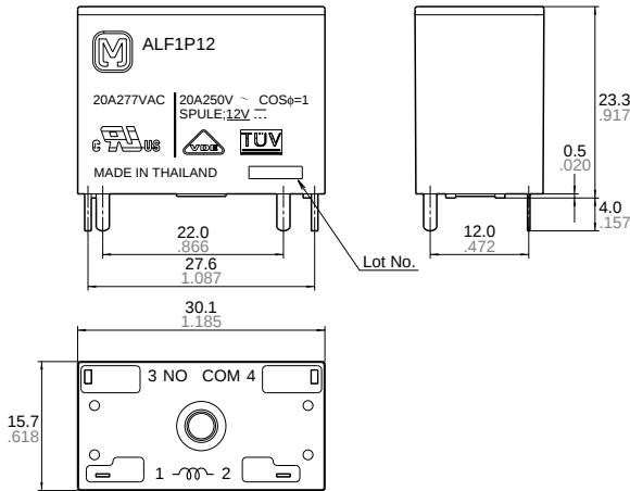
External dimensions
