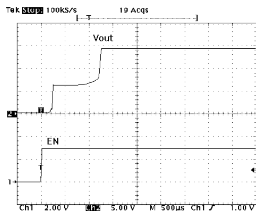
Figure 19 : Enable Time
