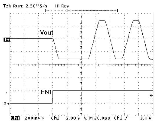
Figure 16 : Tone Enable
