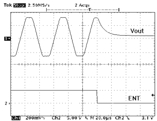
Figure 17 : Tone Disable
