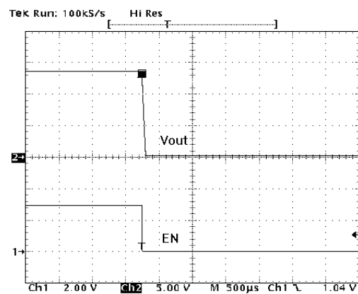
Figure 20 : Disable Time
