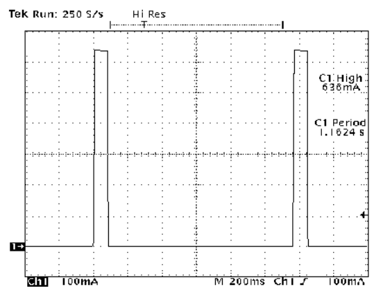
Figure 15 : Dynamic Overload protection ( I_{SC} vs Time)
