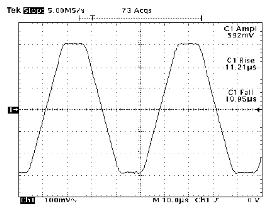
Figure 18 : 22KHz Tone
