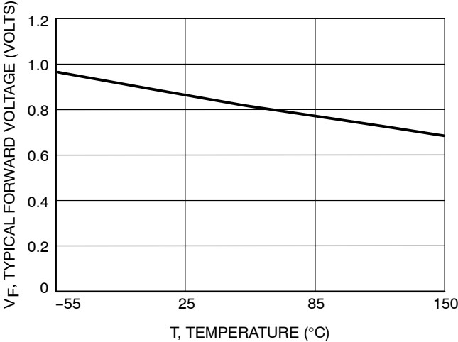
Figure 7. Forward Voltage
