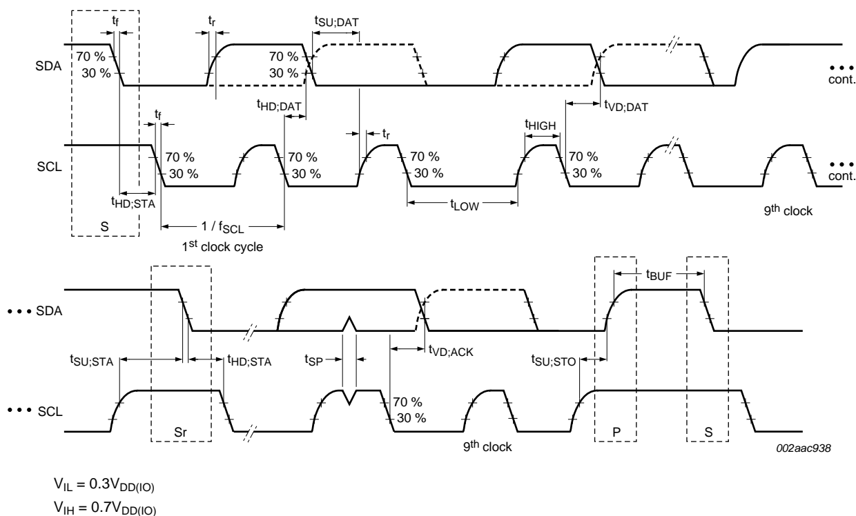
Fig 8. Definition of timing for F/S-mode devices on the I 2 C-bus
