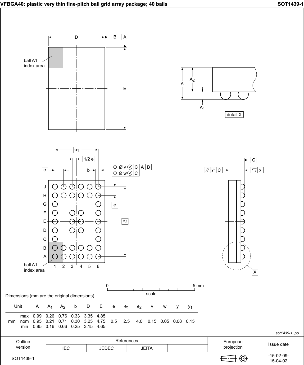
Fig 9. Package outline SOT1439-1 (VFBGA40)
