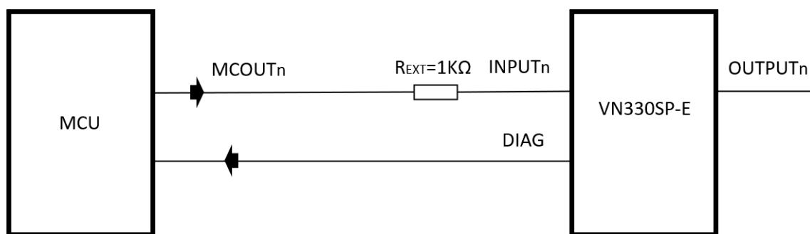
Figure 8. Driving circuit
