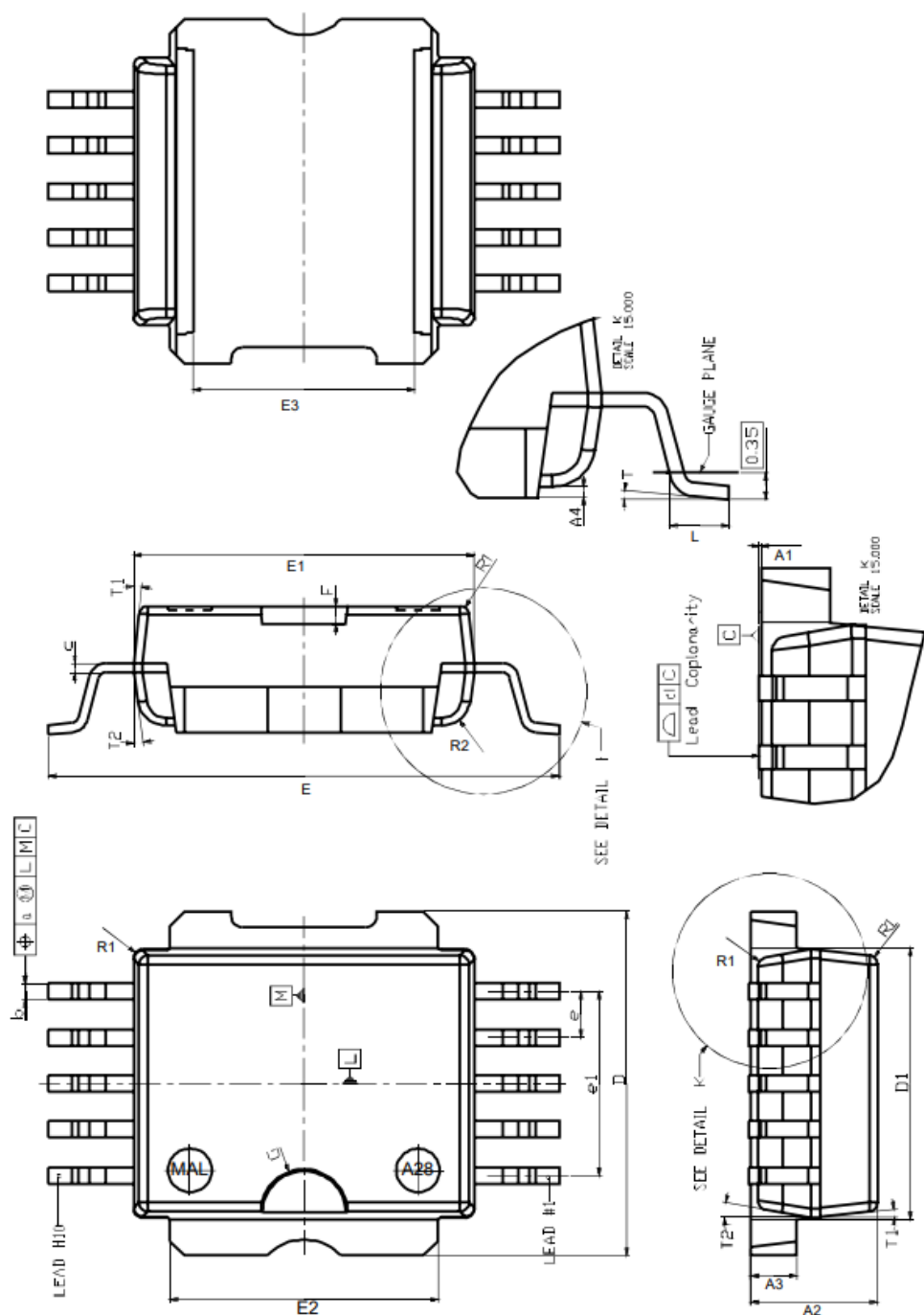
Figure 9. PowerSO-10 package outline
