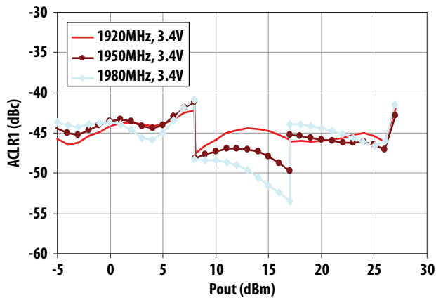
Adjacent Channel Leakage Ratio 1 vs. Output Power
