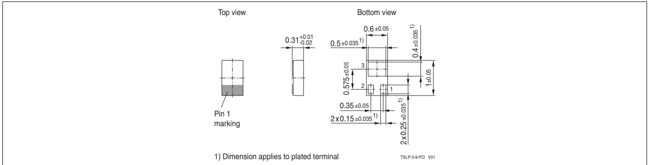
Figure 7-1 Package Outline
