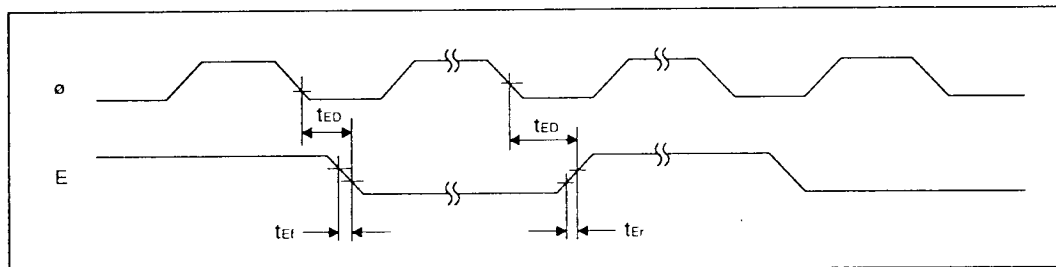
Figure 20-11 E Clock Timing
