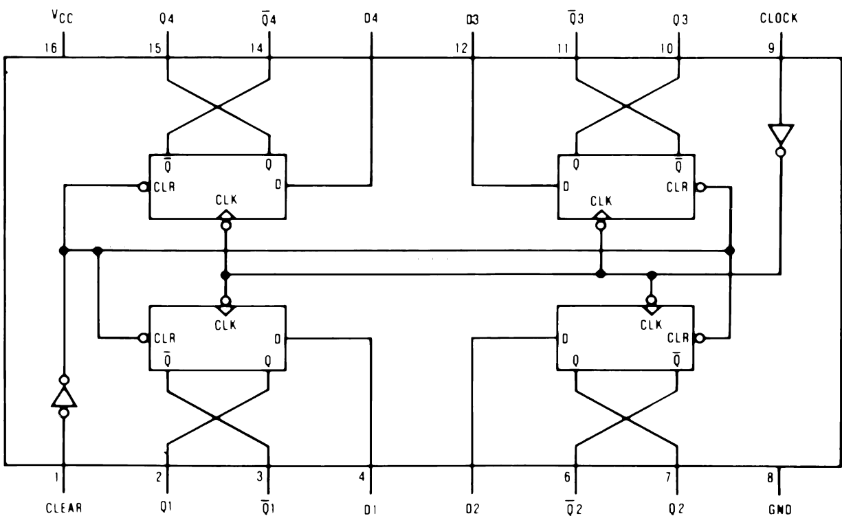
DM74ALS175
