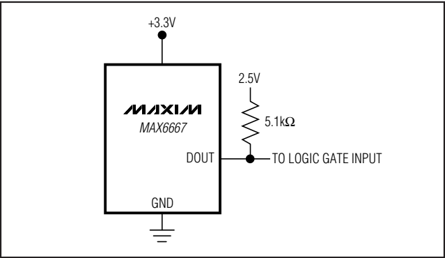
Figure 4. Low-Voltage Logic
