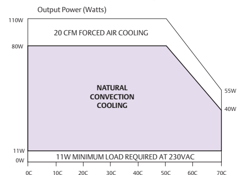
DERATING CURVE (See Notes 9, 10)
