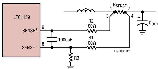
Figure 7. Suppressing Burst Mode Operation
