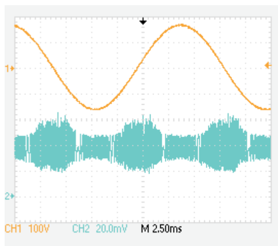
Figure 10. LED Output Voltage Ripple, Full Load, No Dimmer ( V_{IN} = 115 VAC, CH1 = V_{OUT} )
