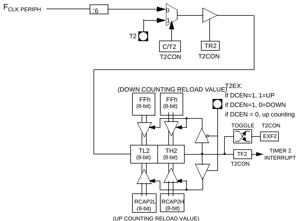
Figure 28. Auto-Reload Mode Up/Down Counter (DCEN = 1)
