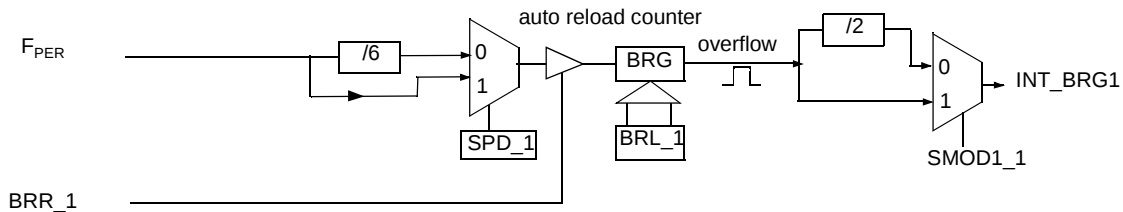
Figure 43. Internal Baud Rate generator 1
