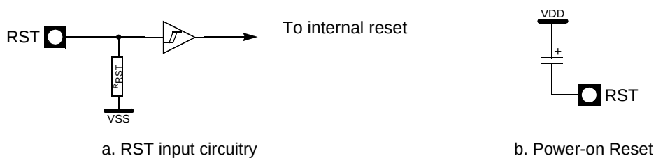
Figure 69. Reset Circuitry and Power-On Reset
