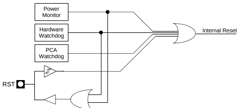
Figure 68. Reset schematic
