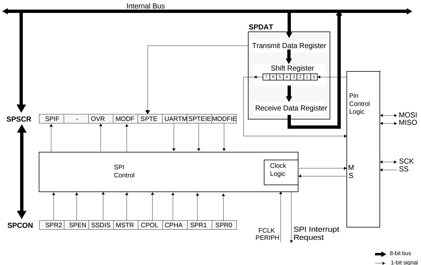
Figure 57. SPI Module Block Diagram
