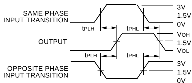
Propagation Delay
