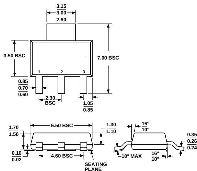
Figure 23. 3-Lead Small Outline Transistor Package [SOT-223] (KC-3)
