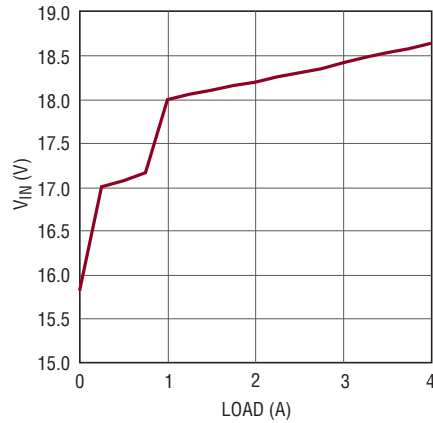
Minimum V_{IN} vs Load, V_{OUT} = 15\text{V}
