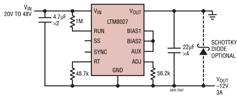
-12V V_{OUT} Positive-to-Negative Converter
