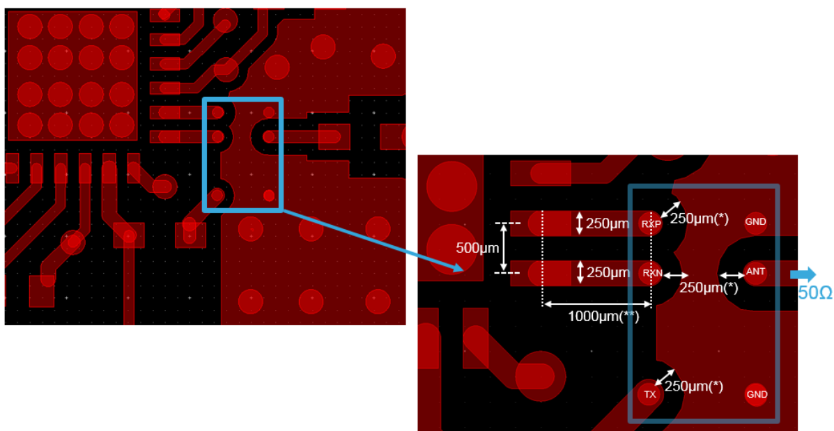
Figure 12. Recommended balun land pattern
