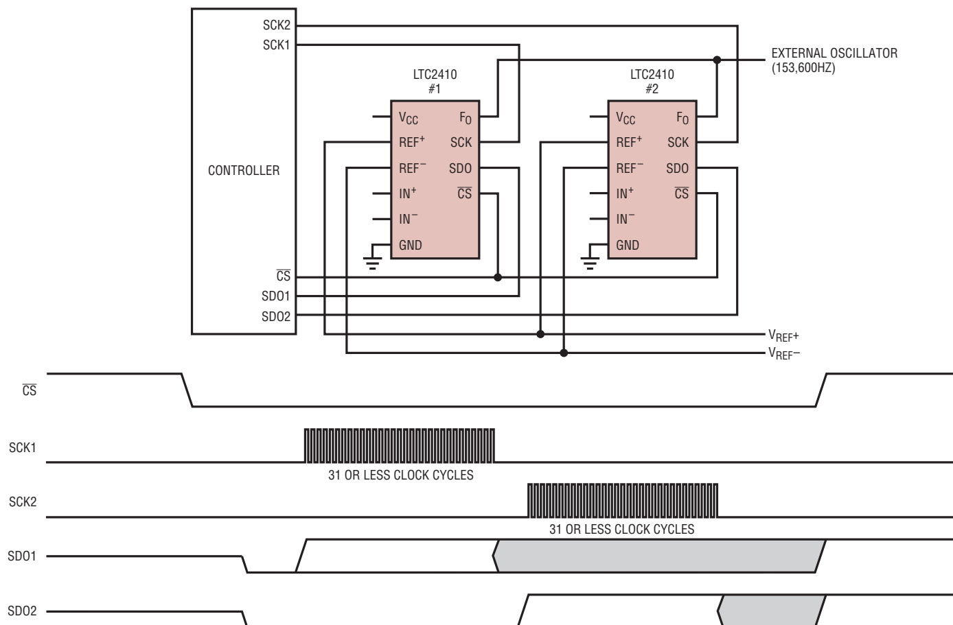
Figure 45. Synchronous Conversion—Extendable
