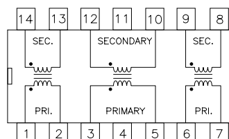
Triple Schematic
