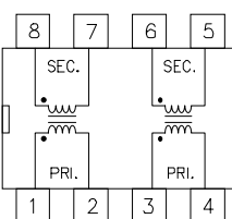
Dual Schematic
