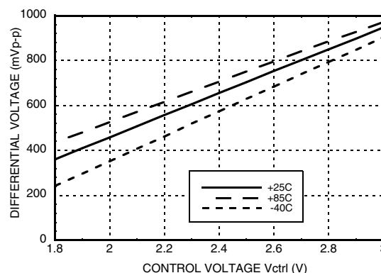
Differential Output Swing vs. Vctrl [1]
