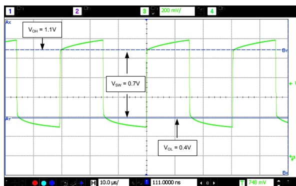
Figure 4. SiT1533AI-H4-D14-32.768 Output Waveform (10 pF load)
