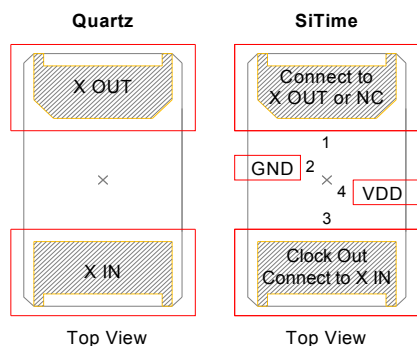
Figure 2. SiT1533 Footprint Compatibility with Quartz XTAL Footprint [6]
