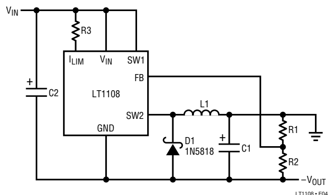
Figure 4. Positive-to-Negative Converter
