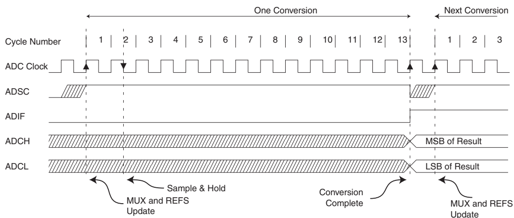
Figure 21-5. ADC Timing Diagram, Single Conversion
