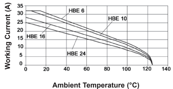
HBE CAGE CLAMP: 2.5 mm 2 (14 AWG)
